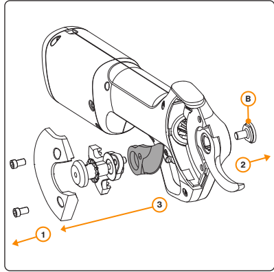
Figure 8. Changing the cutting blade. Follow the sequence of the numbers. 4. Installation in reverse order but make sure that the blade is clearance free when you tighten the blade screws. Check that there is no gap between the cutting and lower (hook) blades.
