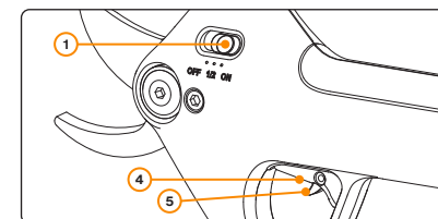
Figure 3: The power switch (1), trigger switch (4) and safety trigger (5).
