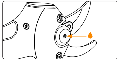
Illustration 5: Smörjhålets placering.
