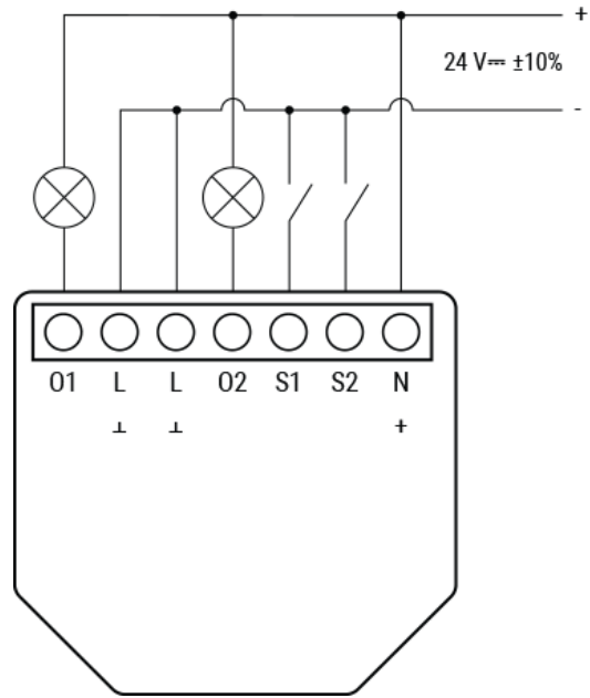
Dual-channel switch mode, DC power supply
