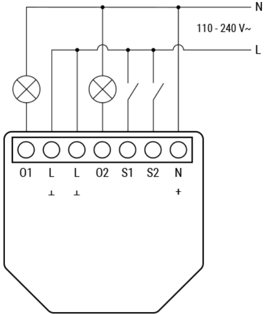
Dual-channel switch mode, AC power supply
