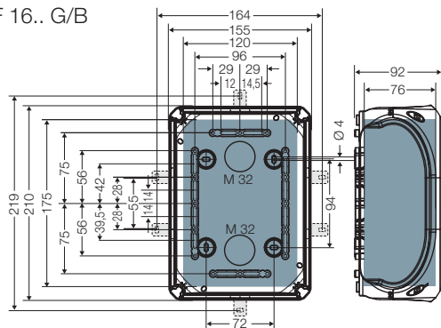
KF 16.. G/B
