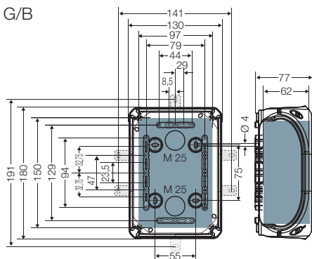
KF 16.. G/B
