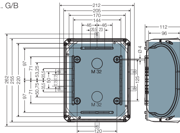
KF 35.. G/B
