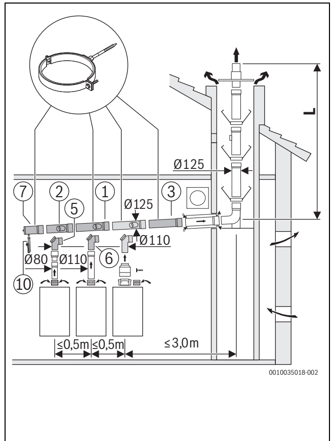
11 DN125 - DN125
