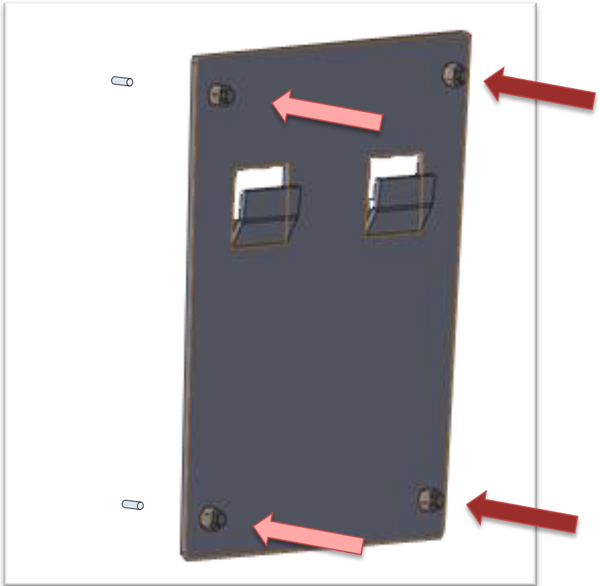
Illustration3. Fastening of the bracket
