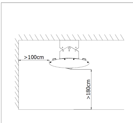
Ceiling installation:
