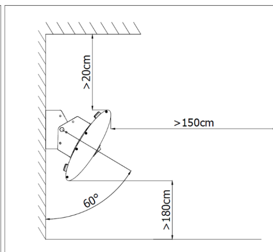
Wall installation:
