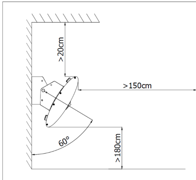
Wand montage:
