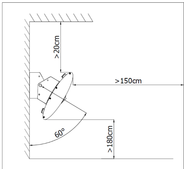
Wandmontage:
