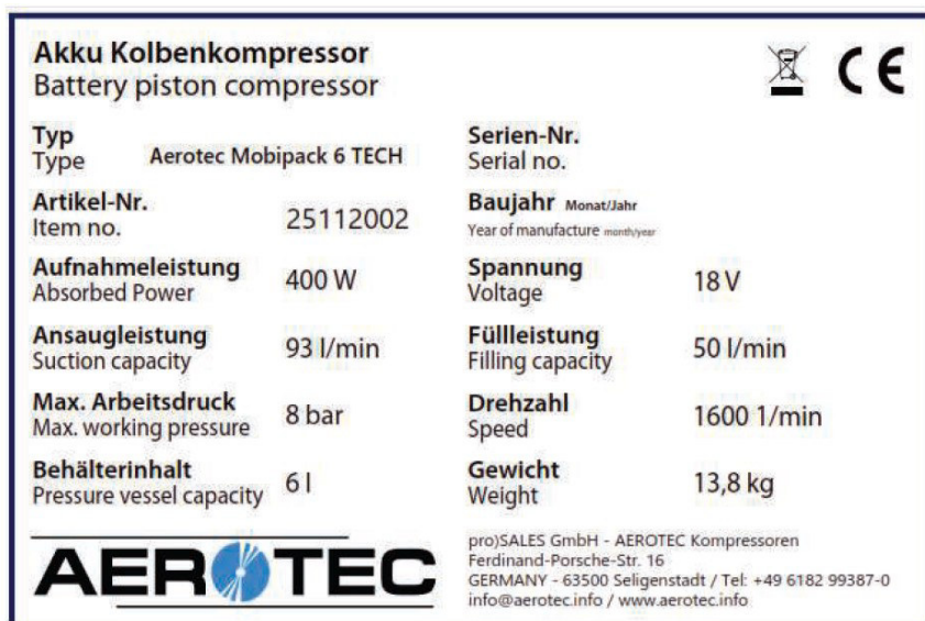
Abb.2-1: Typenschild Mobipack Mobipack 6 TECH
