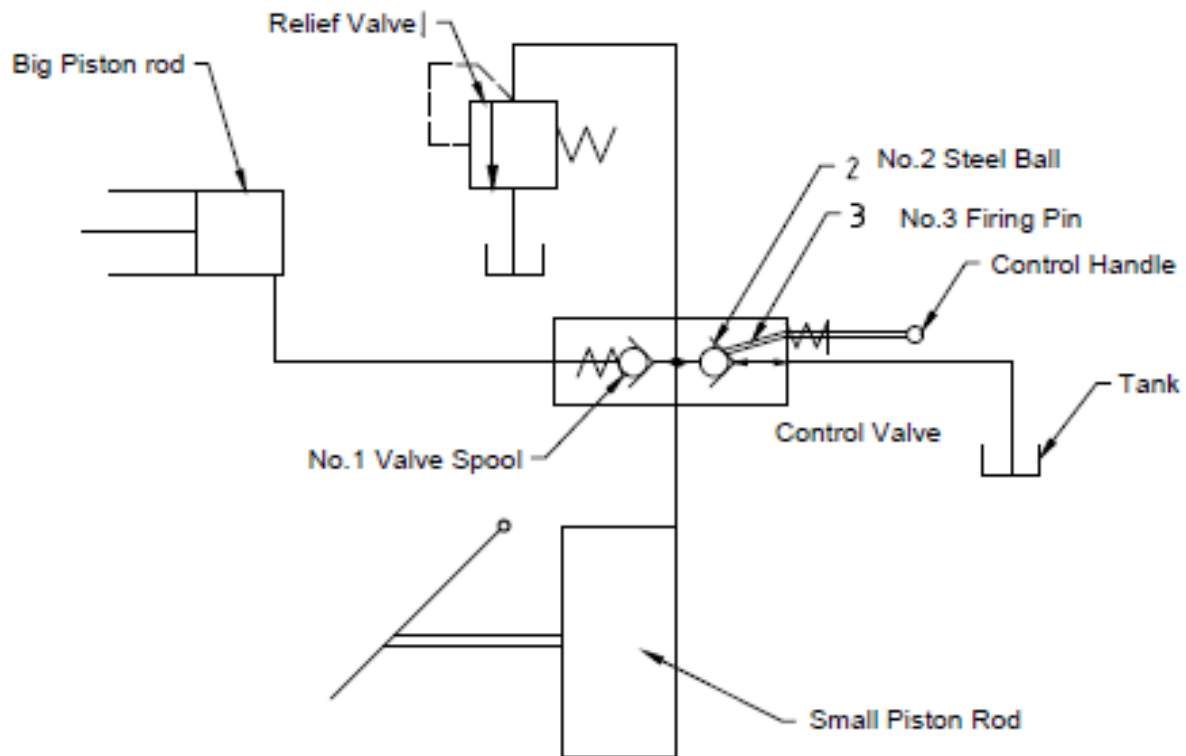
Abb.10-1: Hydraulikplan
