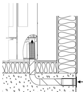
Through floor and foundation
