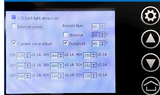
The power curve adjustment menu
