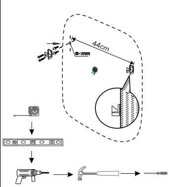
2 Vertical hanging option
