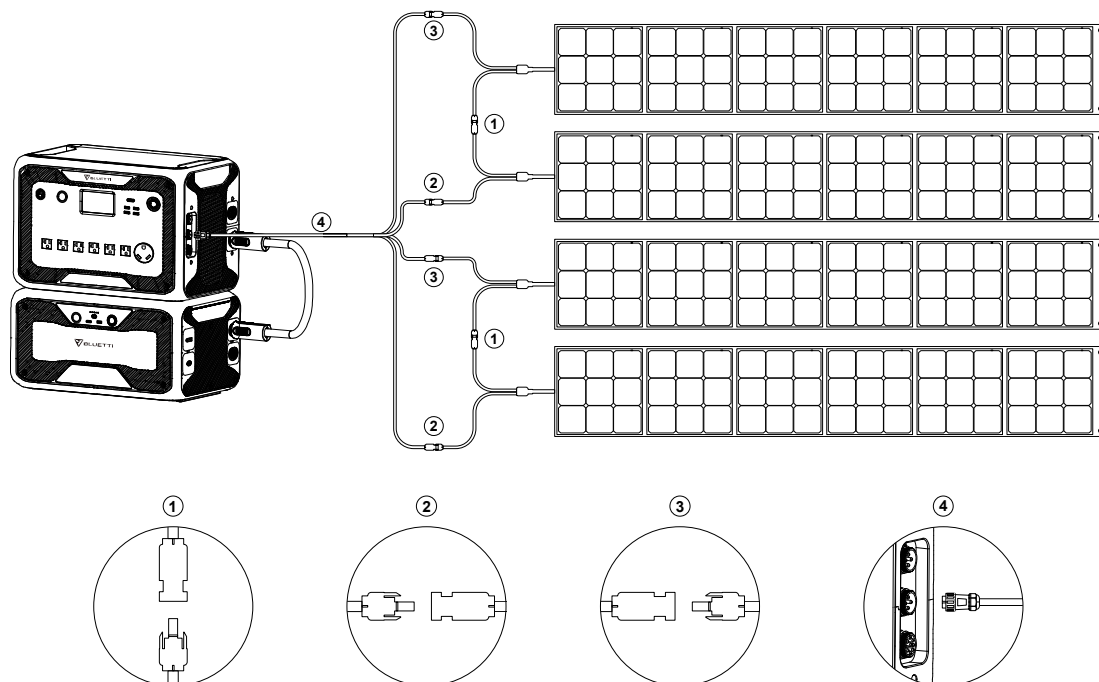
( Easy steps to solar charging )
