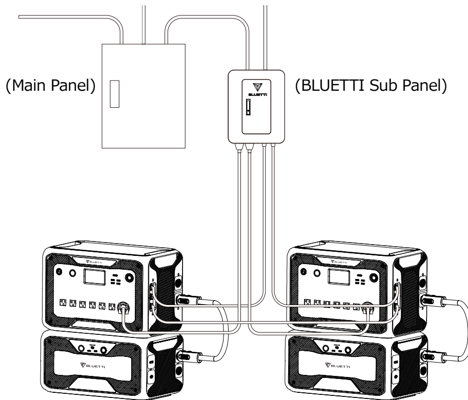
( AC300 grid-tie home power back-up system )
