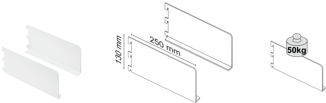
Book brackets
