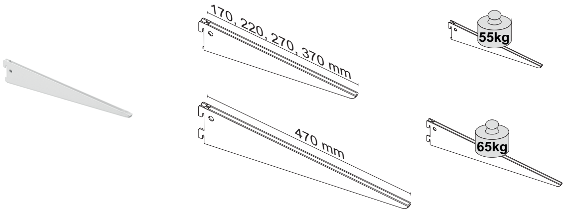
double slot brackets
