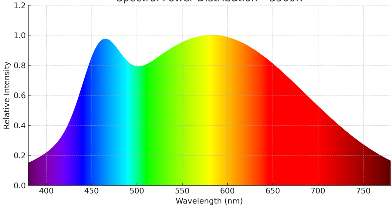
Spectral Power Distribution - 3500K
