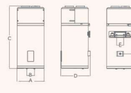
*Dimensions (mm)
