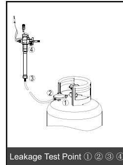
Leakage Test Point ① ② ③ ④
