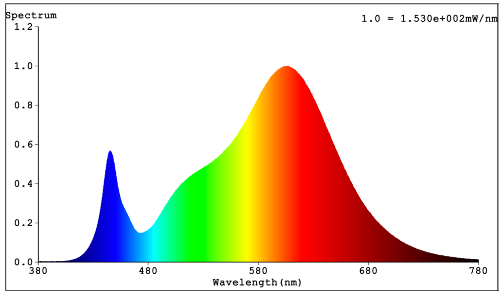
Data 3: Spectral power distribution for light source of YZ-2019-48V-90:
