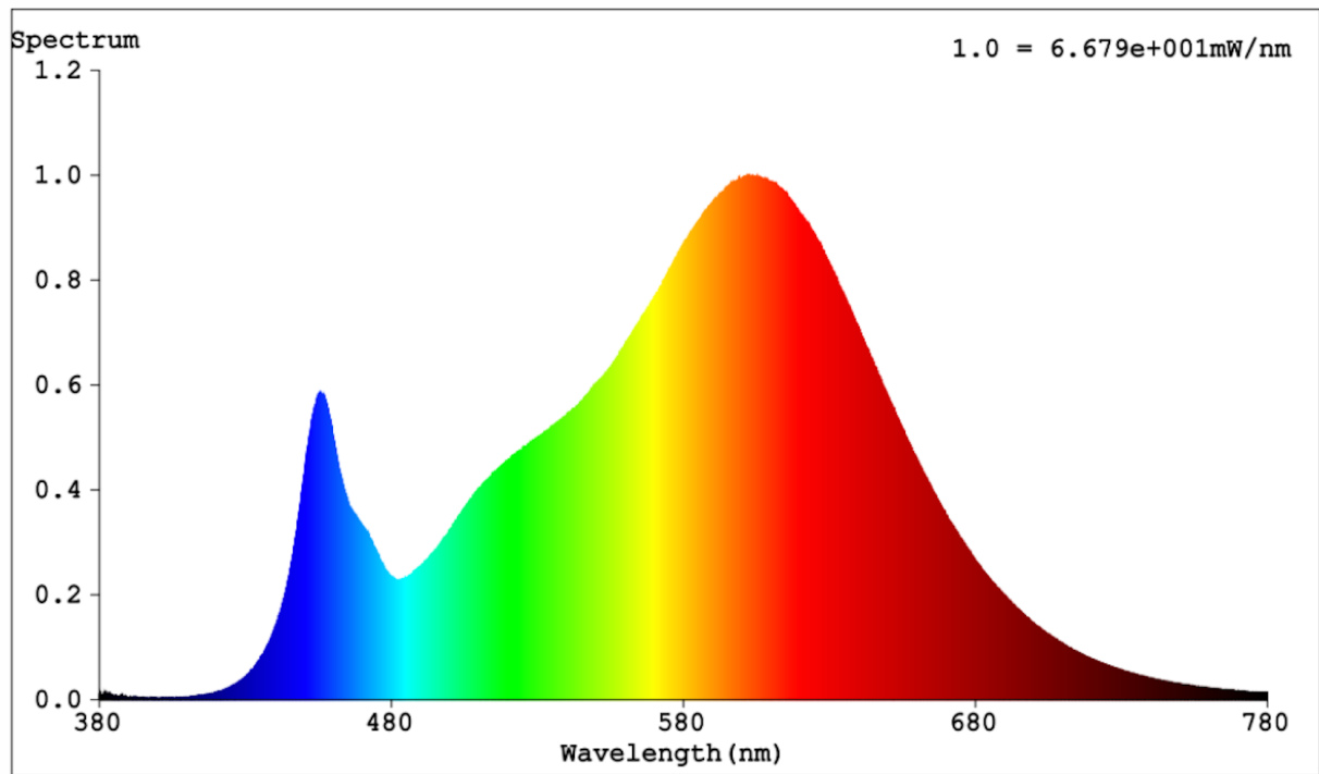
Data 3: Spectral power distribution for light source of C31993NK.25W.DM (9626811) :
