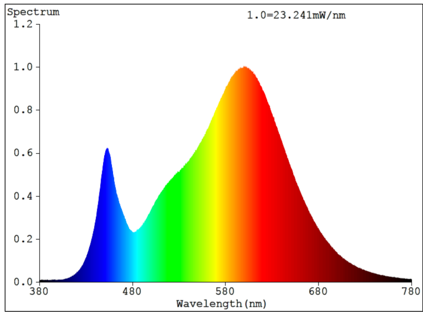
Spectrum of sample 1#
