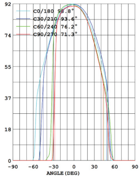
LUMINOUS INTENSITY DISTRIBUTION
