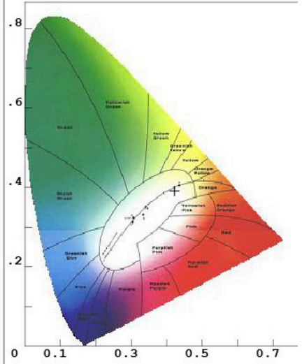
y CIE1931 Chromaticity Diagram
