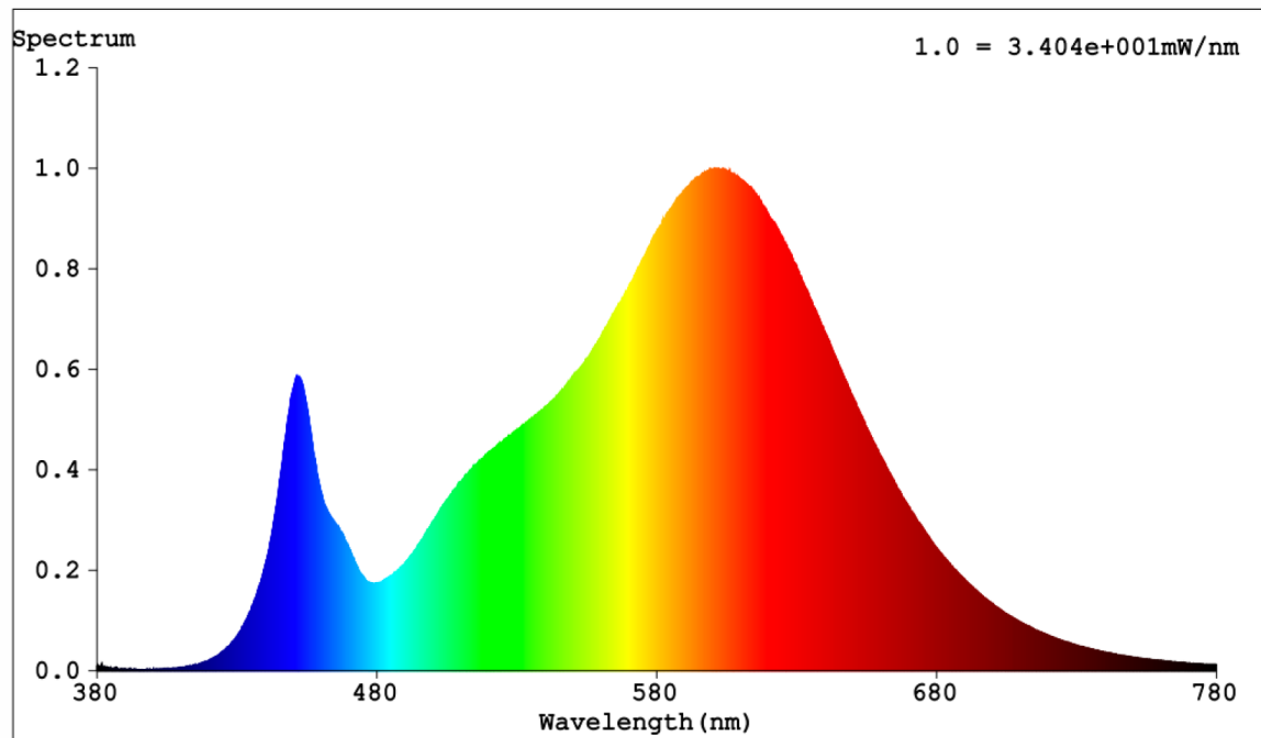
Data 3: Spectral power distribution for light source of 2x165-6B6C-2835:
