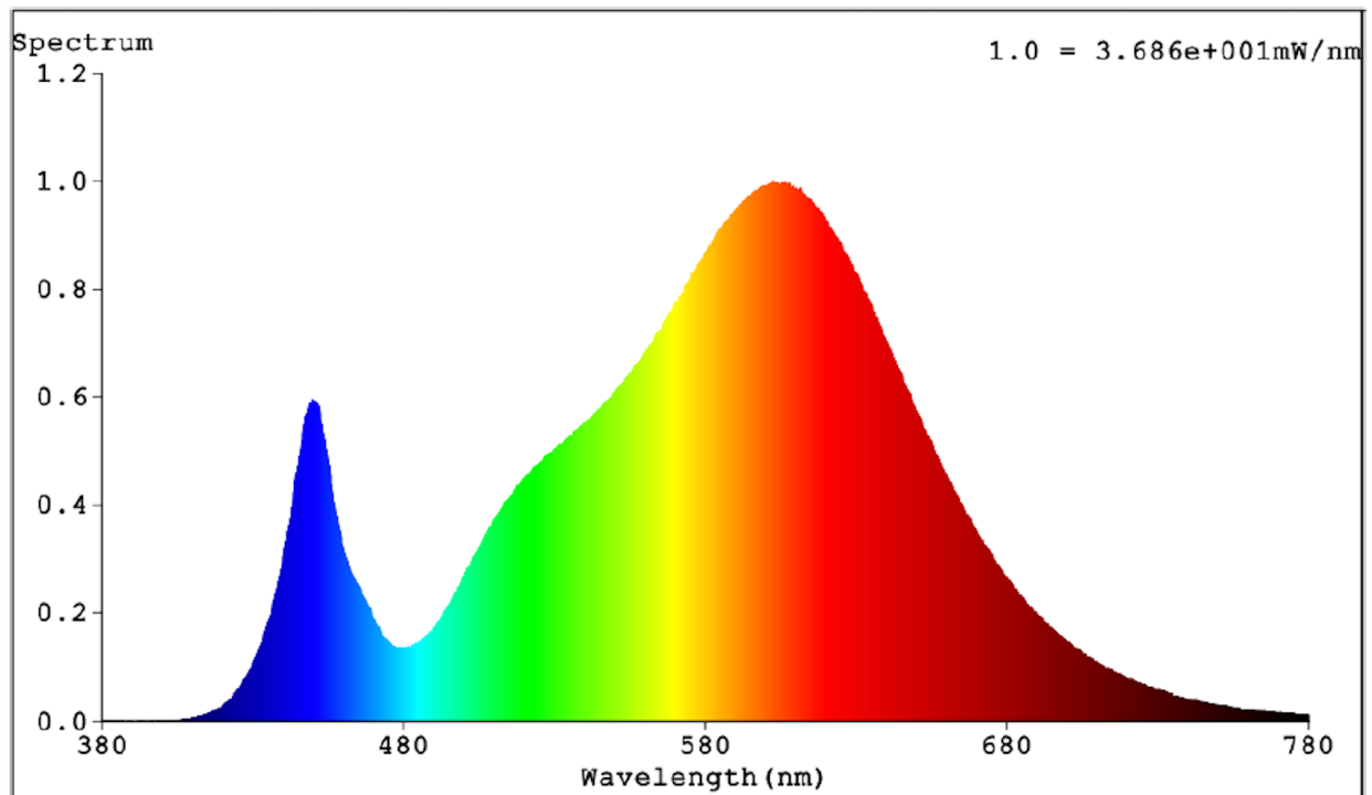
Data 3: Spectral power distribution for light source of WS143 A1 7C14B 24V 670mA:
