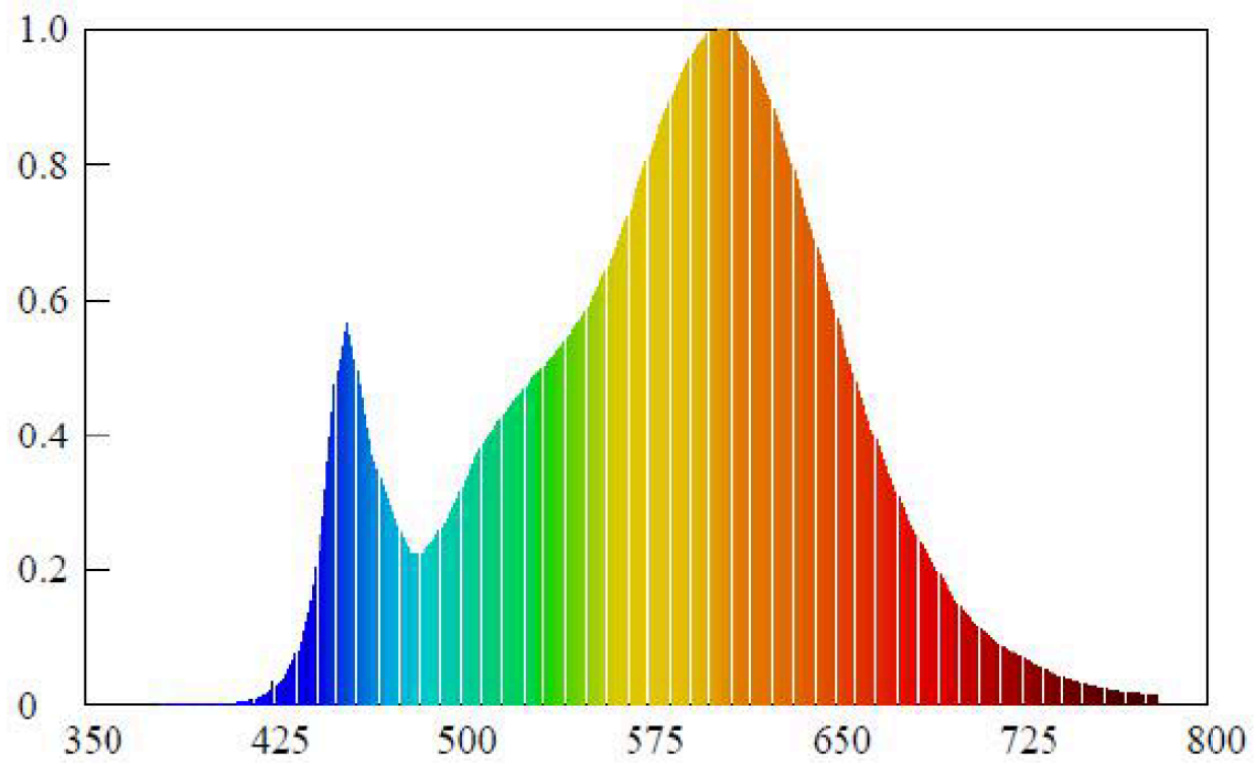
Spectral power distribution (For model CL1512-18-E 18W)
