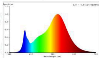
Spectrum
