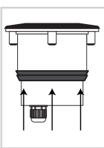
GASKET INSTALLATION
