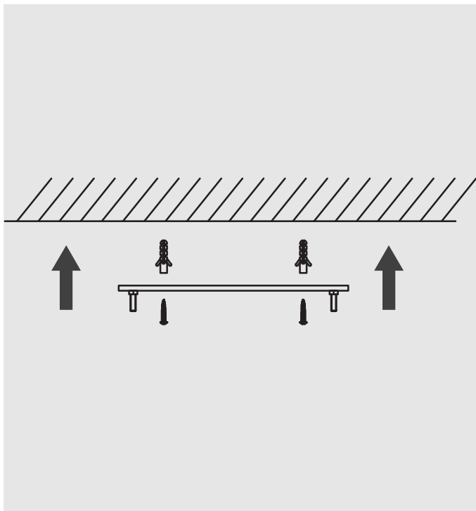
① Fix the mounting bracket to the ceiling.
