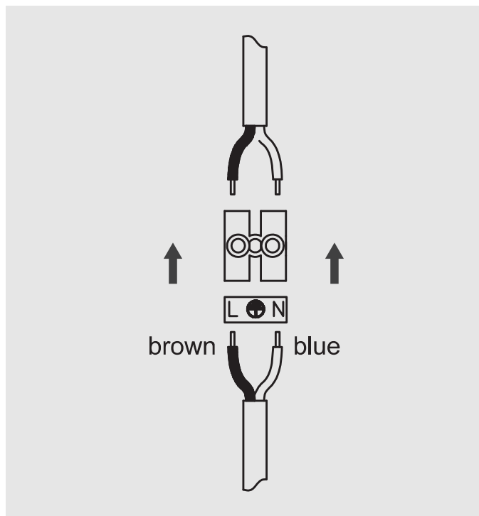
② Connect the power cord to the lamp.
