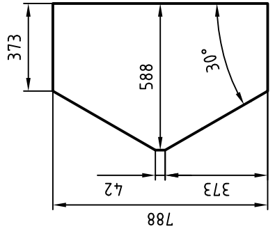
Detail Z
