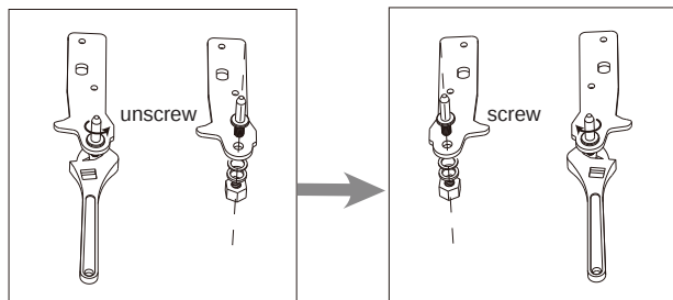
Step 6: Unscrew and remove the bottom hinge pin, turn the bracket over and replace it.
