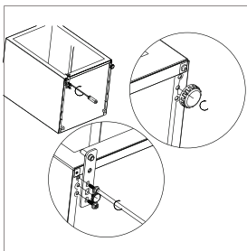
Step 6: Reassemble lower suspension and reattach height-adjustable feet.
