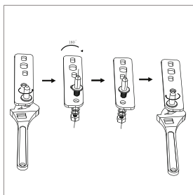
Step 5: Unscrew lower suspension and remove pin. Rotate suspension 180° and reattach pin.
