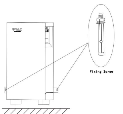
Fig.6-3 Fix the Battery to the Wall
