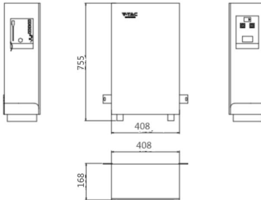
Fig. 5-1 Product Dimensions
