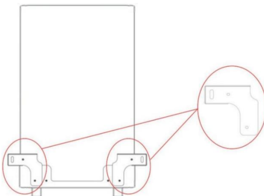
Fig.6-1 Fix the Brackets to the Battery
