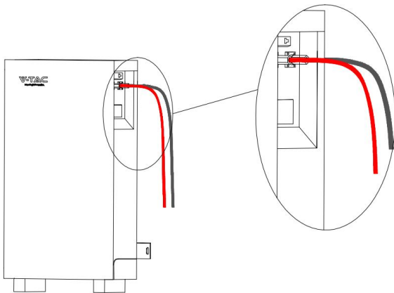
Fig.6-5 Communication Cable Connection Diagram
