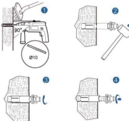
Fig.6-2 Fix the screws to the wall
