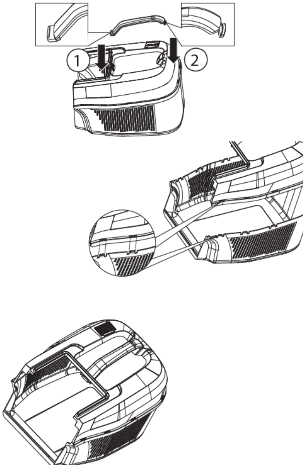
Assembling grass catcher
