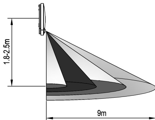
Height of installation: 1.8-2.5m
