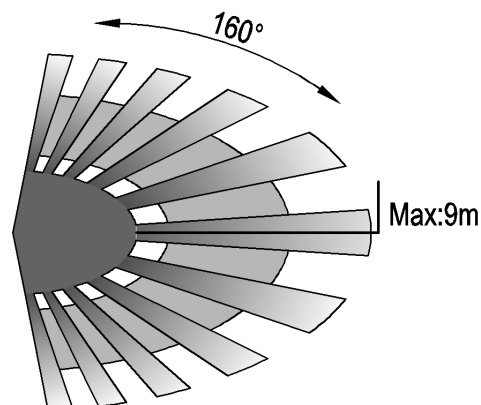
Detection Distance: Max. 9m
