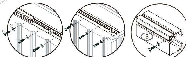
Screw mounting position
